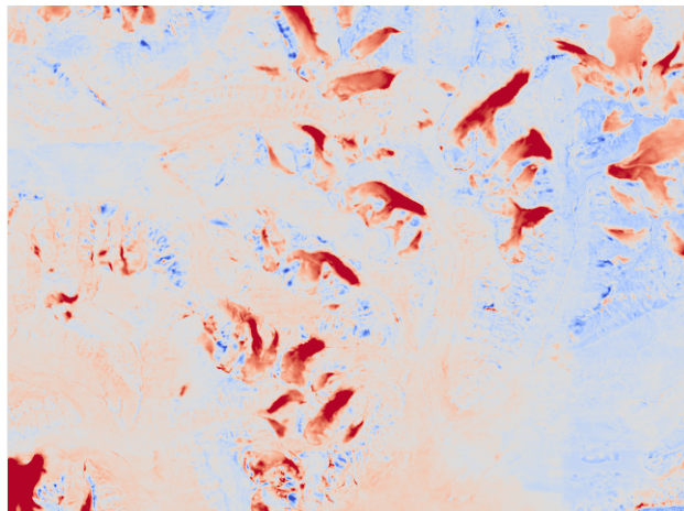
After coregistration. NMAD=2.5 m
