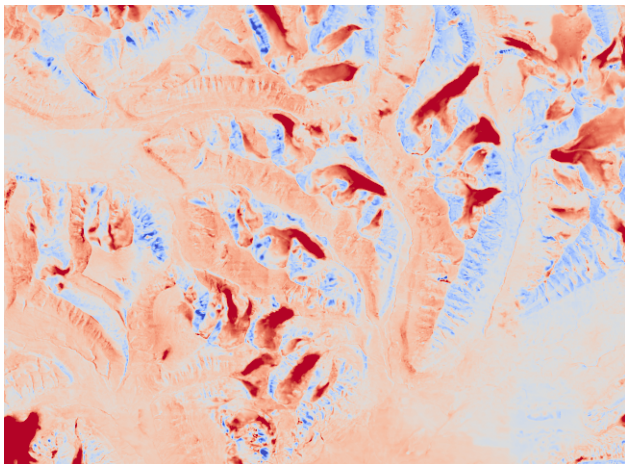
Before coregistration. NMAD=3.4 m
