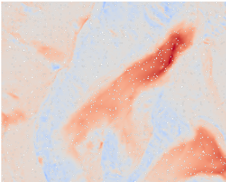
dDEM with random voids
