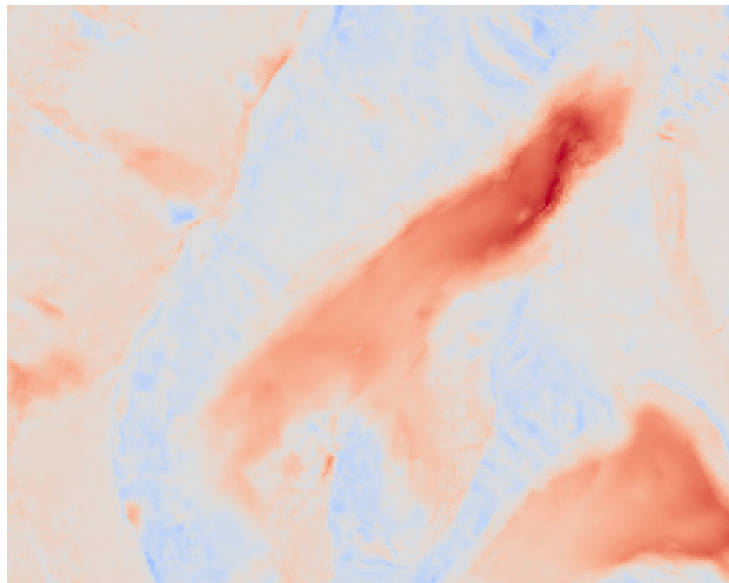
Linearly interpolated dDEM
